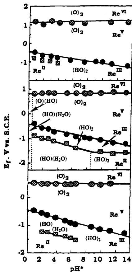
Figure 9. Pourbaix diagrams for t\text{-(O)}_2\text{Re}(\text{Me}_2\text{py})_4^+ (top), t\text{-(O)}_2\text{Re}(\text{py})_2(\text{dmap})_2^+ (middle), and t\text{-(O)}_2\text{Re}(\text{pyrrpy})_4^+ (bottom) in 50:50 \text{CH}_3\text{CN}/\text{water} .
