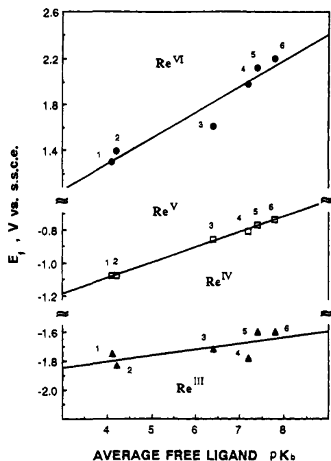
Figure 11. Formal potentials in acetonitrile for t\text{-}(\text{O})(\text{MeO})\text{ReL}_4^{3+/2+/1+} vs free ligand (L) basicity. Key to ligands: (1) pyrpy, (2) dmap, (3) py + dmap, (4) MeOpy, (5) Me 2 py, (6) Me-py.
