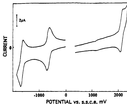
Figure 10. Cyclic voltammogram (sweep rate = 1 V/s) for t\text{-(O)}(\text{MeO})\text{Re}(\text{MeOpy})_4^{2+} in acetonitrile with 0.1 M TBAPF 6 as electrolyte.
